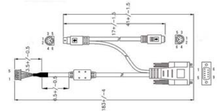
Connect with RS232C Cable (CB-SXR00)
