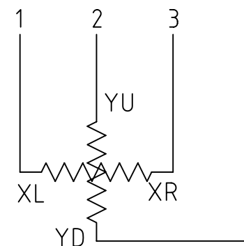
PIN ASSIGNMENT
