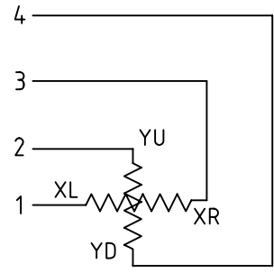
PIN ASSIGNMENT
