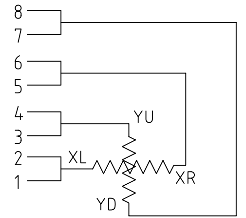
PIN ASSIGNMENT
