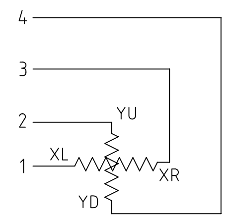
PIN ASSIGNMENT
