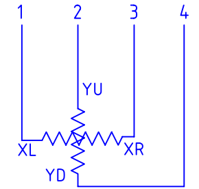
PIN ASSIGNMENT
