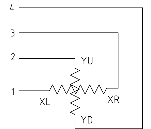
Pin Assignment
