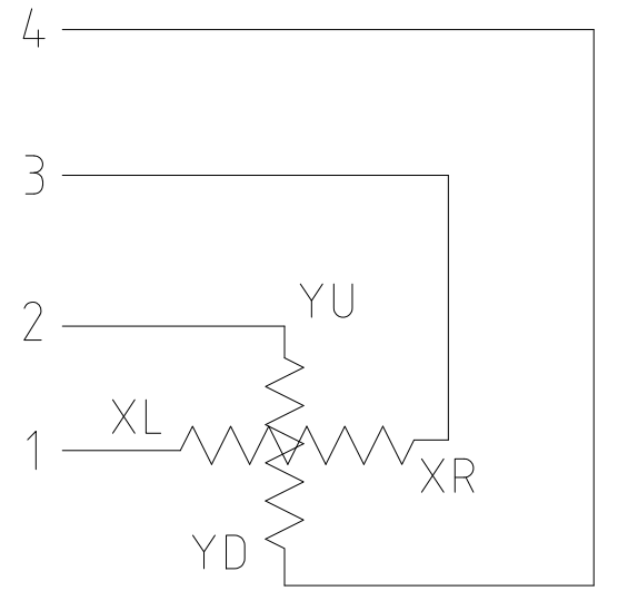
Pin Assignment
