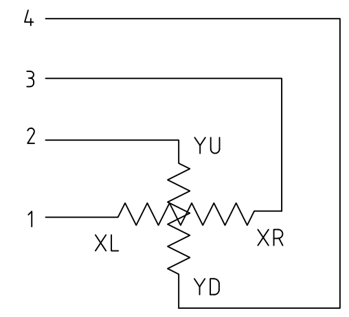
Pin Assignment
