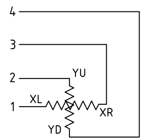
Pin Assignment
